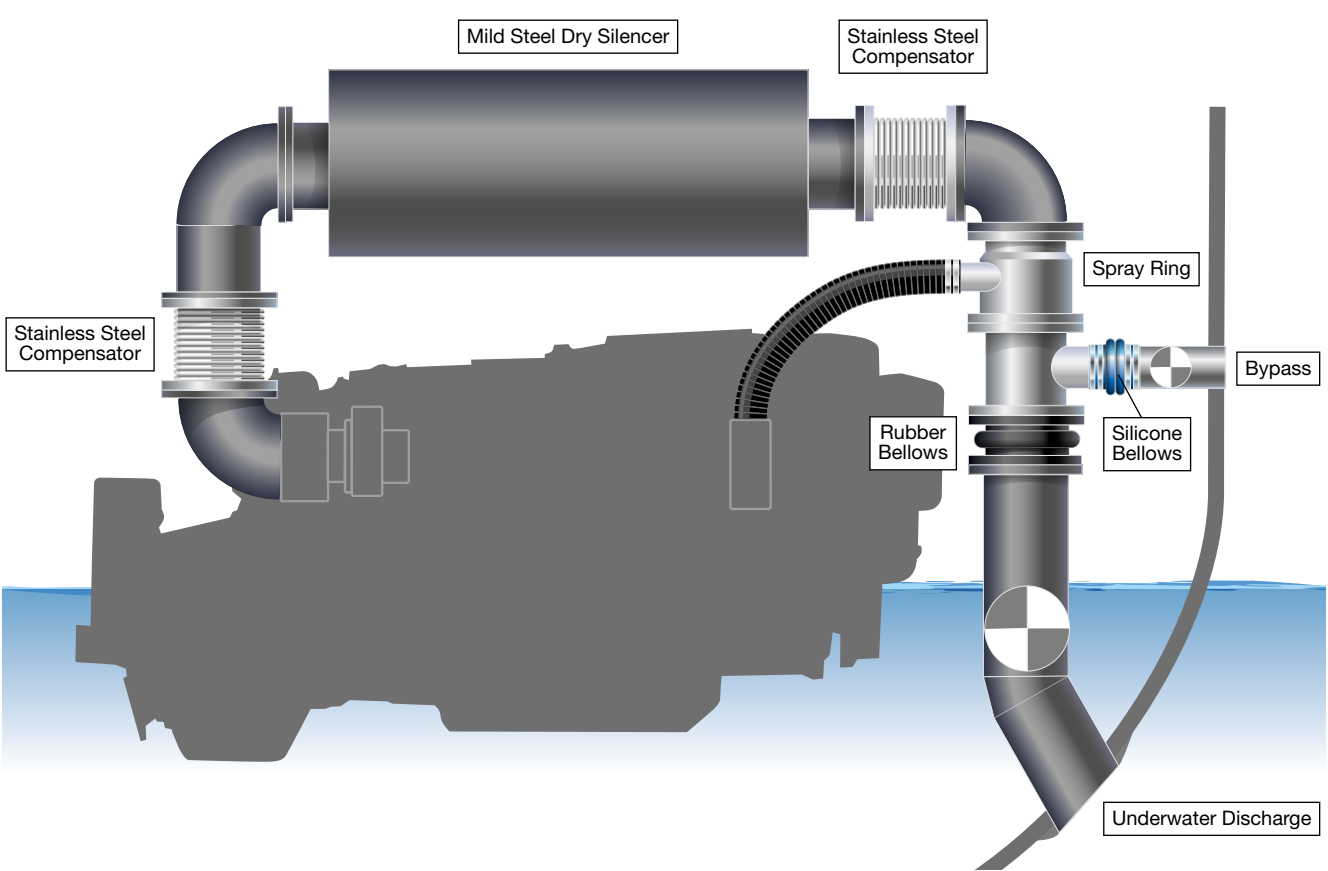
Dry Silencer to Spray Ring with Bypass and Underwater Discharge
