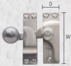
Ball End Fastener D1095 W (single arm) x D (mm): 65 x 20 W (single arm) x D (in): 2 9/16 x 25/32
