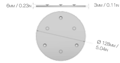
SCREW-FIXING PLATE
