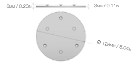
SCREW-FIXING PLATE
