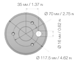
SCREW-FIXING BASE
