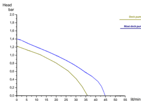
IMPELLER PUMPS
