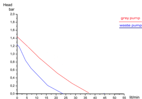
GREY /WASTE WATER PUMP
