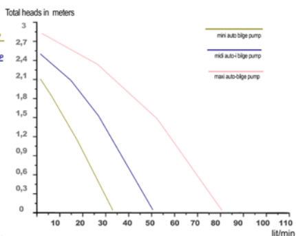
SUBMERSIBLE BILGE PUMPS
