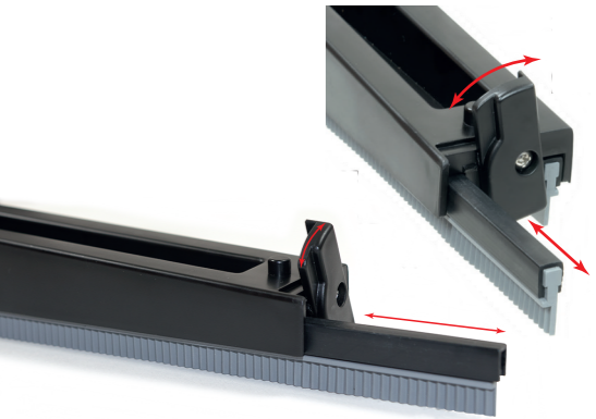
Easy, tool-free change of rubber lips. Item no. 102.115
