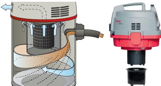
The Illustration shows the patented water separation system
