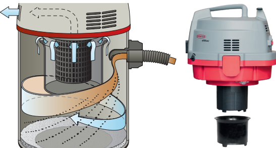
The Illustration shows the patented water separation system
